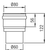
PP adapter
